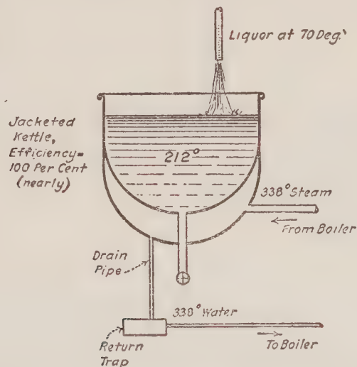
FIG. 5 HEAT TRANSFER IN JACKET KETTLE
